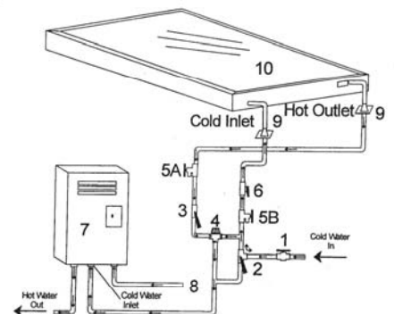
2-Way Schematic Passive Solar Water Heating System With Bosch Tankless
