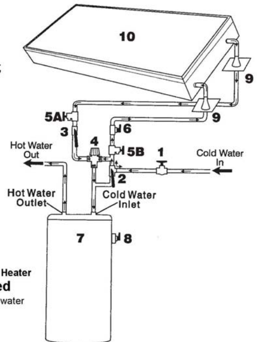
Schematic Passive Solar Water Heating System With Existing Gas Water Heater (backup)
