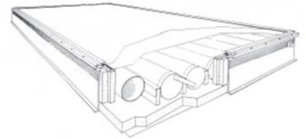
Passive Solar Water Heater Integrated Collector Storage ICS
