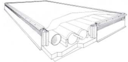
Passive Solar Water Heater Integrated Collector Storage ICS
